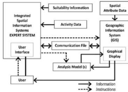
Figure 2: The Expert System Model Procedure [17]
