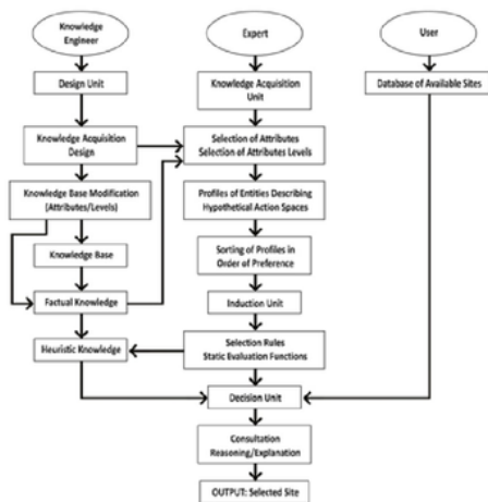
Figure 3: Expert System Schematic Structure For Site Selection [8]
